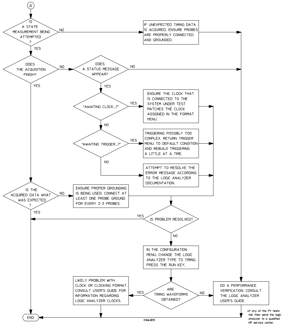
Troubleshooting Flowchart 2
