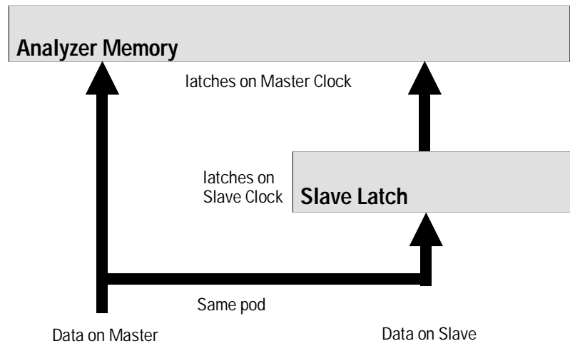
Latching Slave Data in Demultiplex Mode
