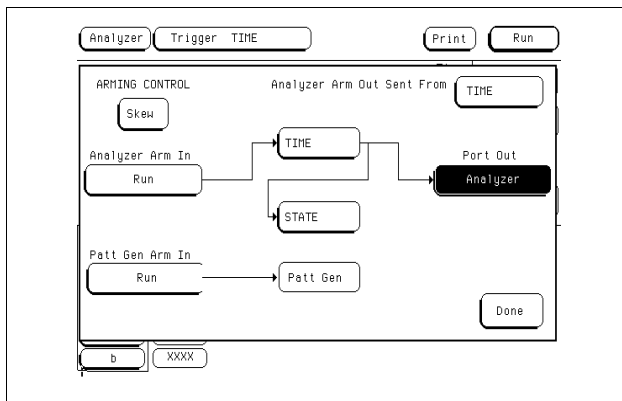
Arming the State Analyzer from the Timing Analyzer
