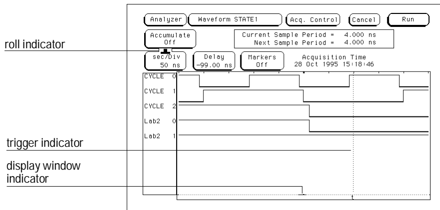
Waveform Display
