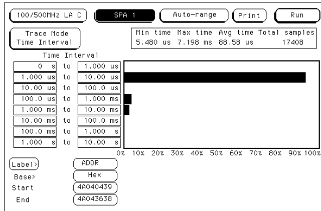
SPA Time Interval
